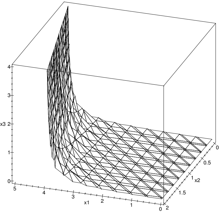
Figure 6.2. The reachability hypersurface of the fed-batch fermenter for initial conditions x_1(0) = 2\frac{q}{7} , x_2(0) = 0.5\frac{q}{7} , x_3(0) = 0.1\frac{q}{7}
